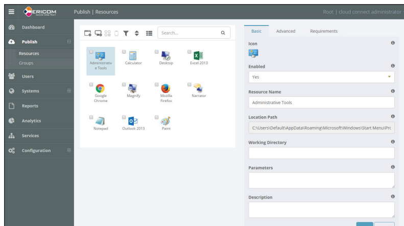
Configure, customize and view all published applications and desktops
